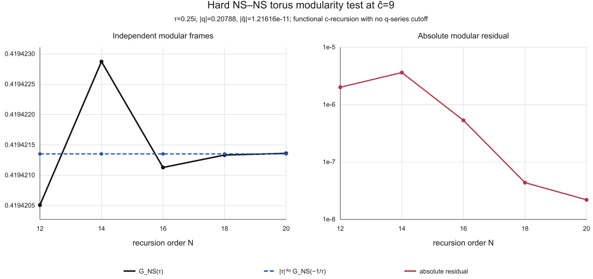
Figure 2: Hard-point recursion-order convergence. Solid black markers show \mathcal{G}_{NS}(i/4) , while dashed blue markers show the independently evaluated 4^{2d}\mathcal{G}_{NS}(4i) . Since |\tilde{q}| = 1.22 \times 10^{-11} , the dashed markers coincide; their common horizontal value is output, not an imposed target. The right panel shows the absolute modular residual.
